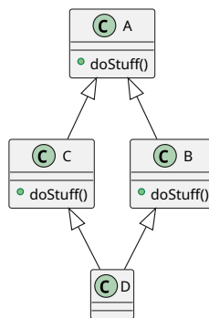
Figure 48: Example of a diamond problem
